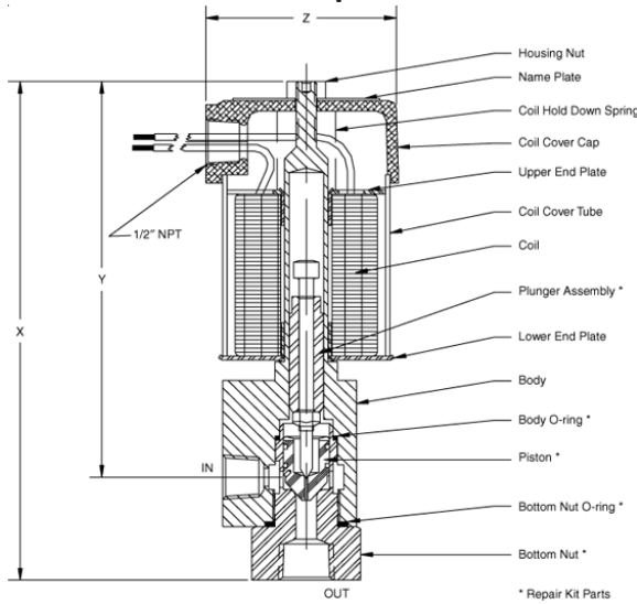
7104 3/8" Valve, shown with a NEMA 1 coil housing
